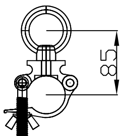
Single Coupler with rigging Eye ST82
