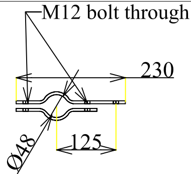
Boom Arm Bracket half length CL30
