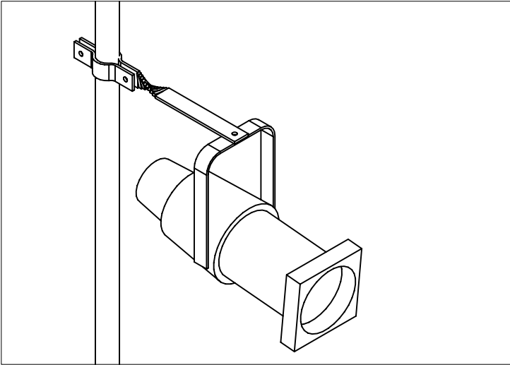
Boom Arm Bracket Straight CL20
